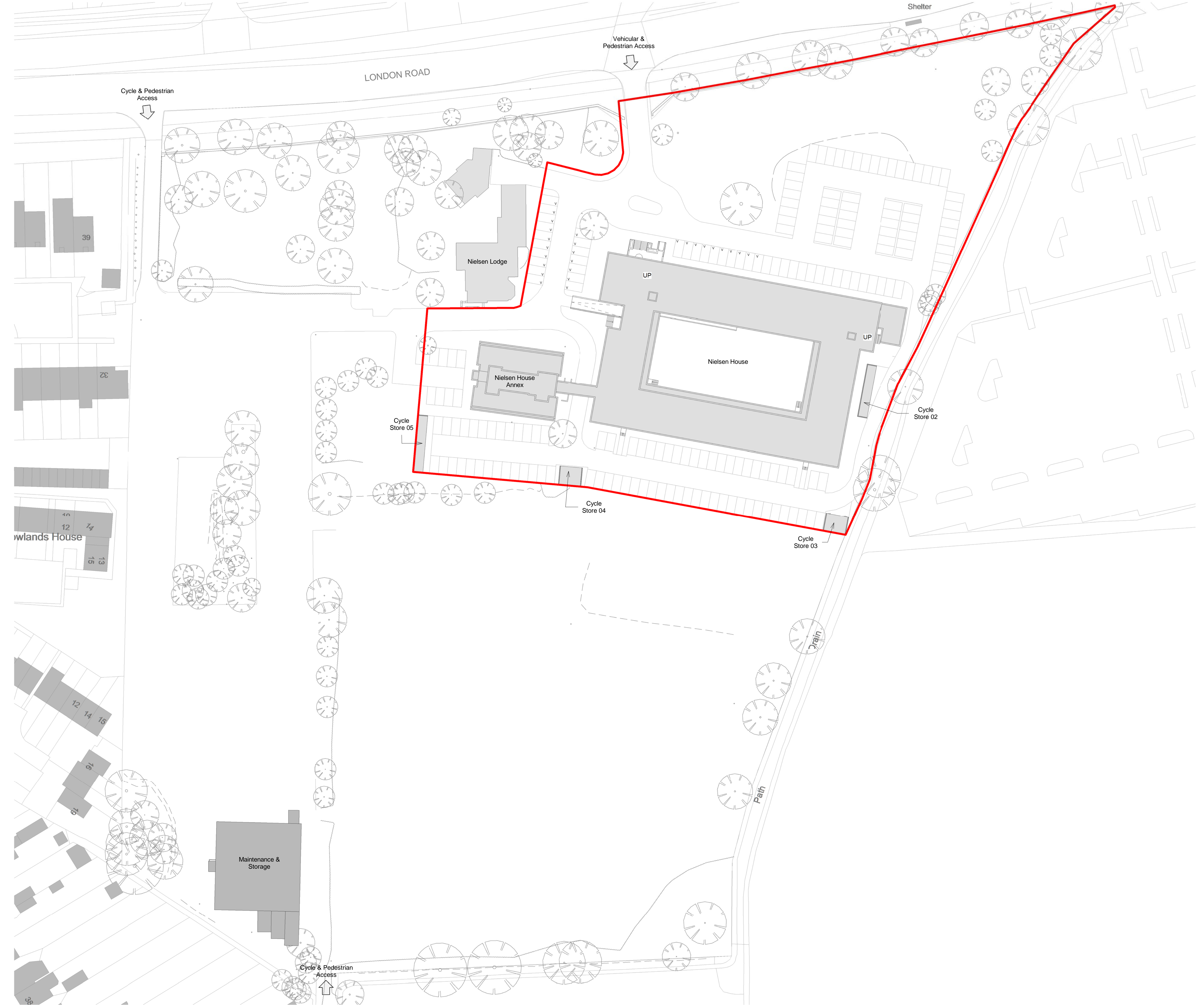
Nielsen House Conversion_Proposed Site Plan 1 : 500
